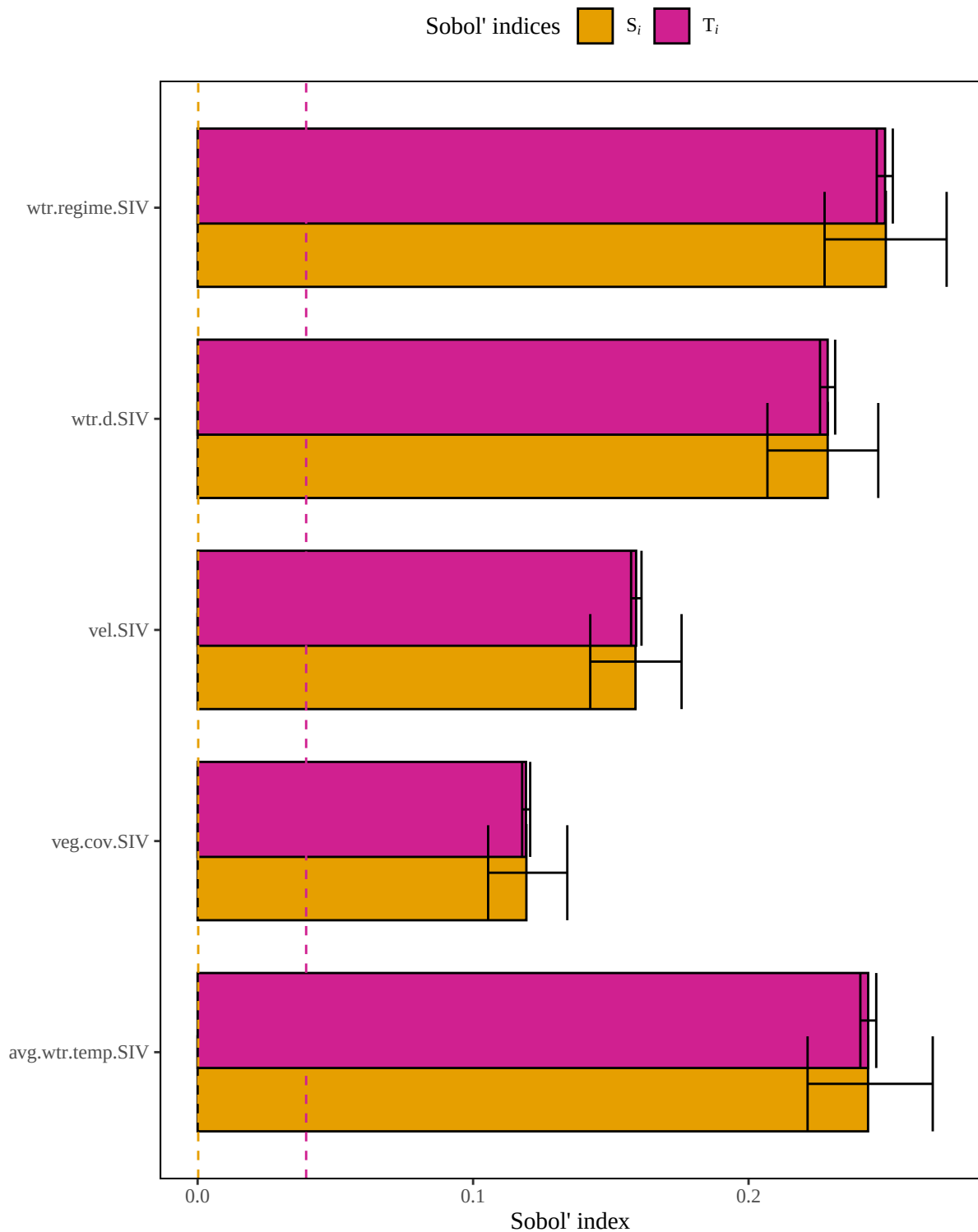
Figure 4. Results of a sensitivity analysis for the sliderturtle model based on an arithmetic mean structure. Dashed lines represent baseline numerical approximation error for S_i and T_i ( i.e. , dummy variables).
