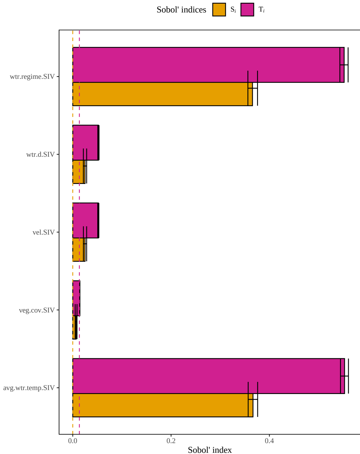
Figure 5. Results of a sensitivity analysis for the sliderturtle model based on a geometric mean structure. Dashed lines represent baseline numerical approximation error for S_i and T_i ( i.e. , dummy variables).
